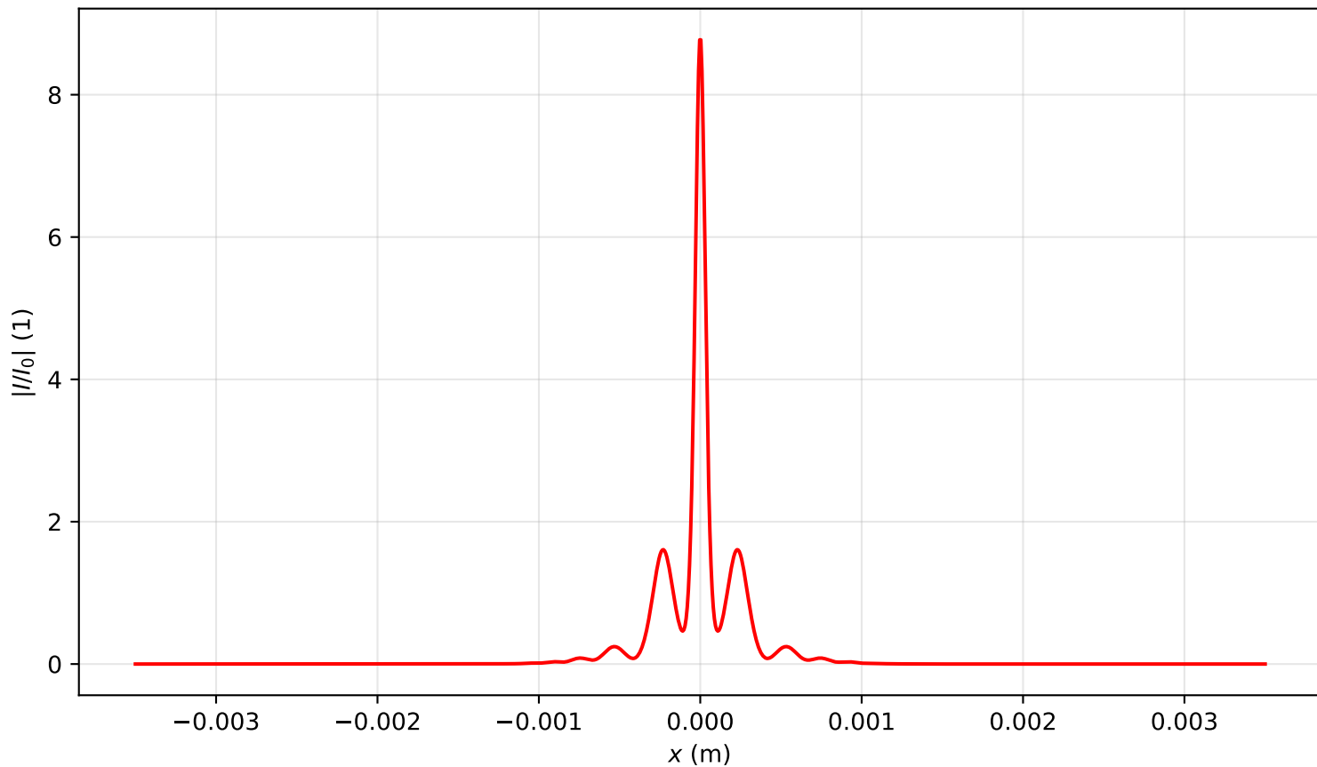
Intensity profile I(x, y = 0, z = 0.478)/I_0 , \text{Pin}=9.0\text{Pcr} , artificial time
